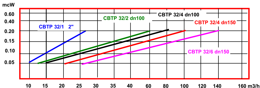
Diagram flow / pressure loss
